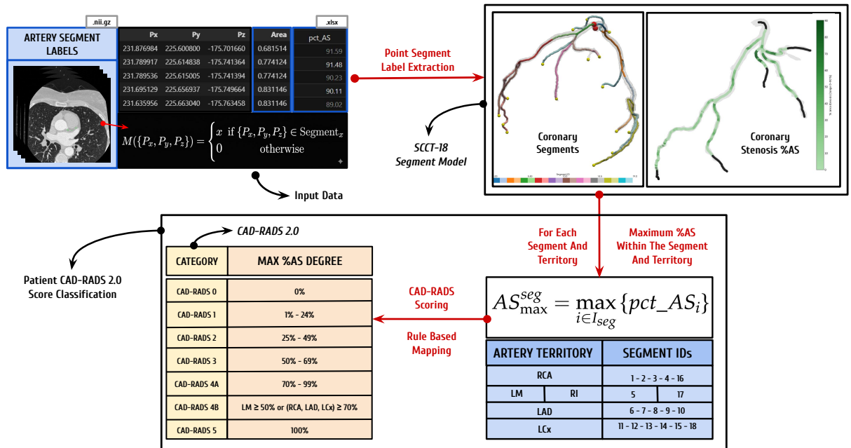
Figure 2.4: Block 3 workflow: segment aggregation based on the SCCT-18 coronary model and automated CAD-RADS 2.0 scoring.
