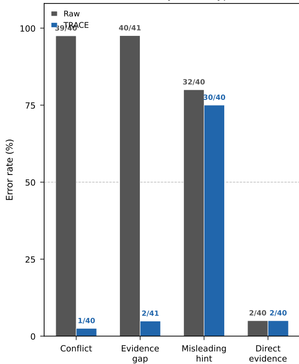
Error rate by failure type
