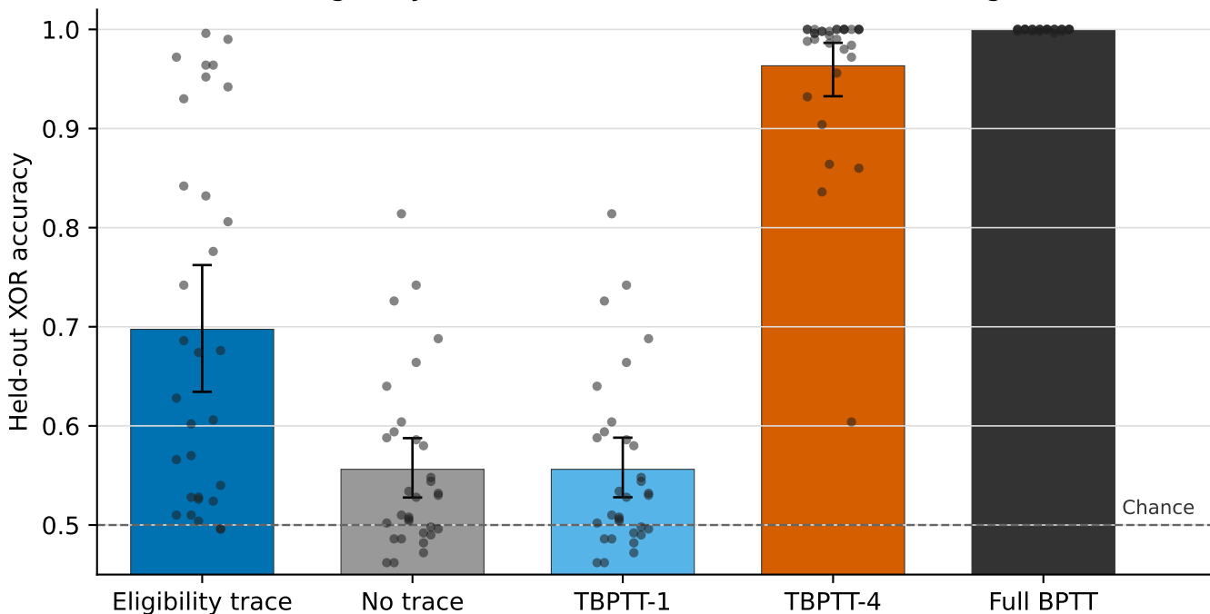
Local eligibility versus truncated recurrent credit assignment
