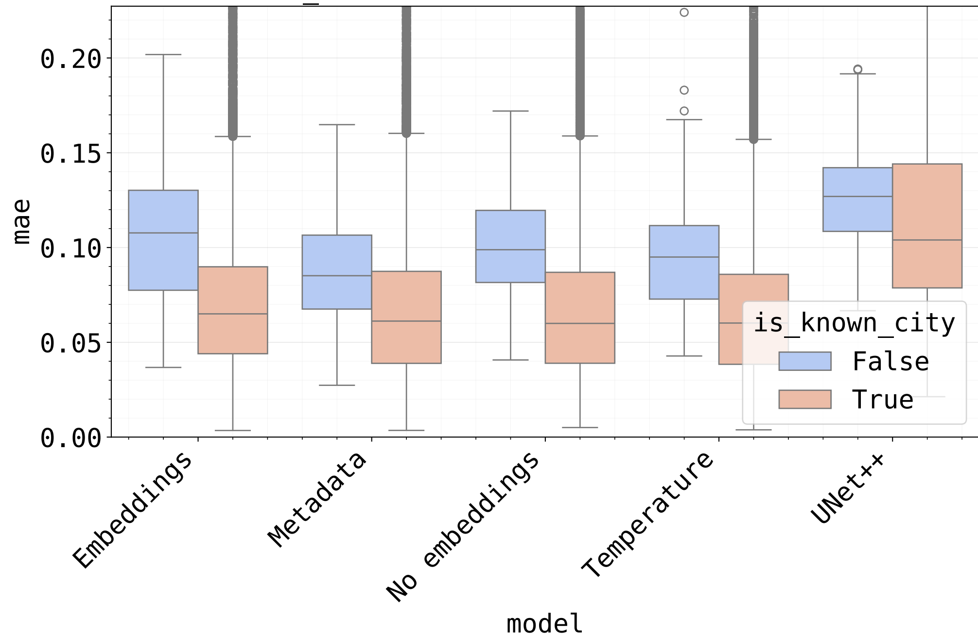
after_ndvi: MAE - Known vs Unknown Cities
