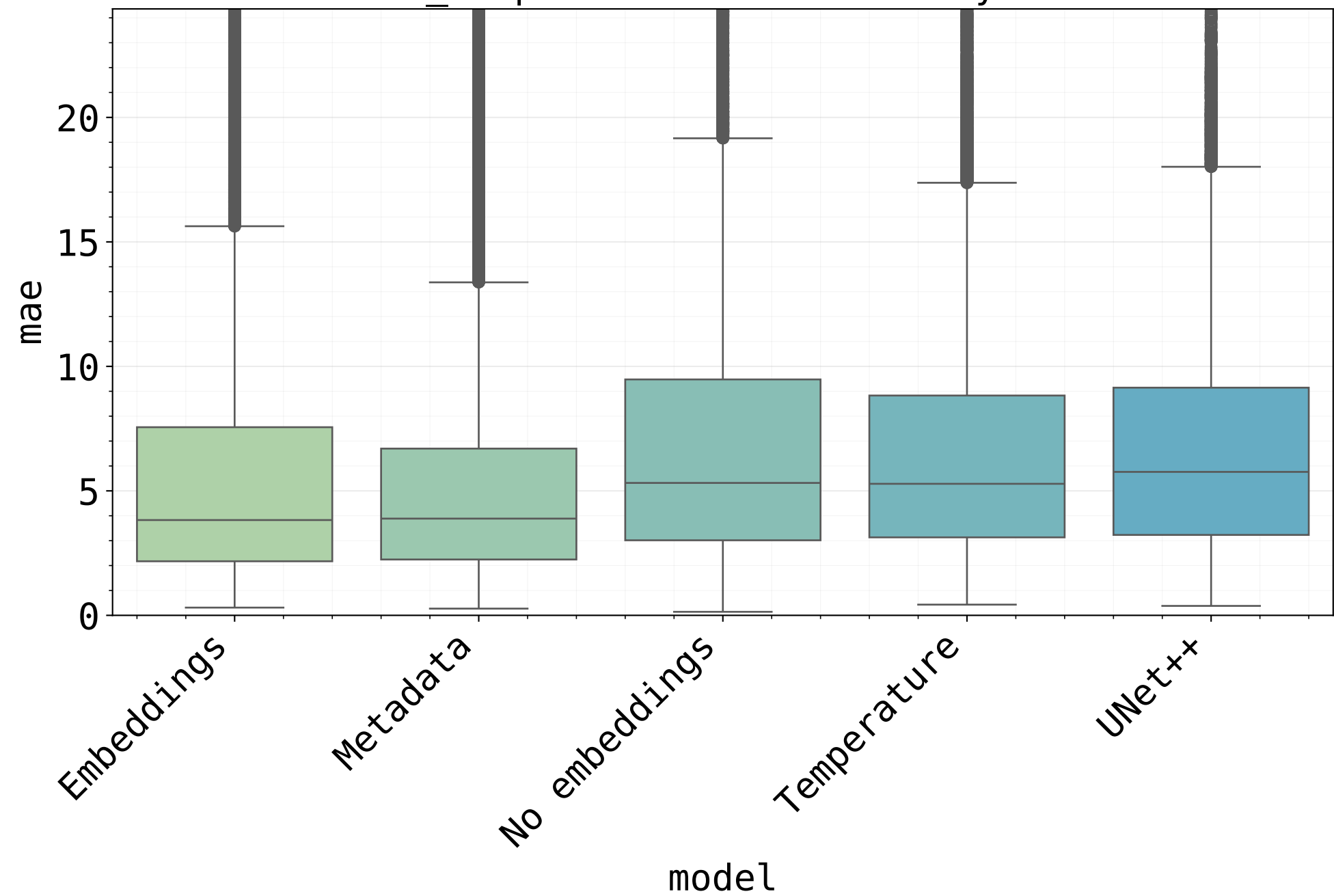
after_temp: MAE Distribution by Model
