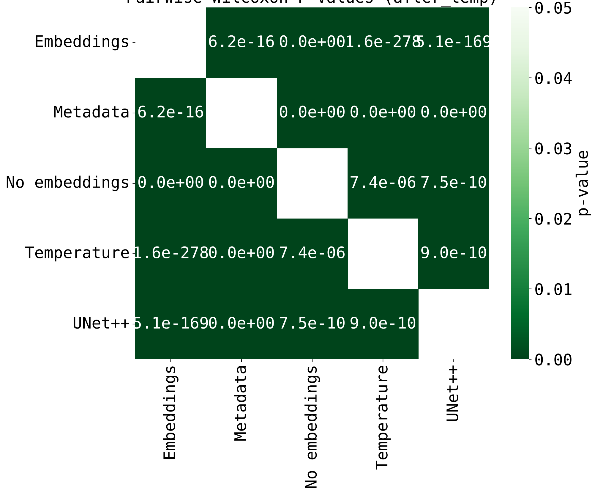
Pairwise Wilcoxon P-Values (after_temp)
