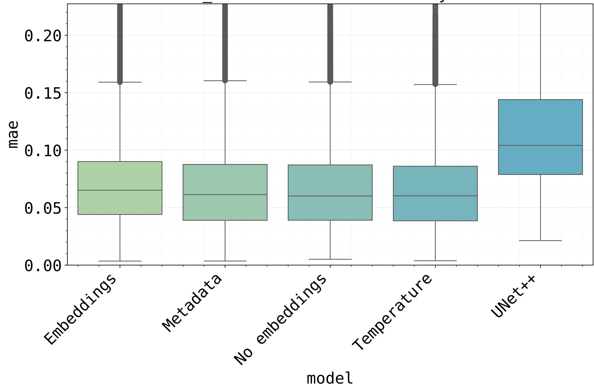
after_ndvi: MAE Distribution by Model
