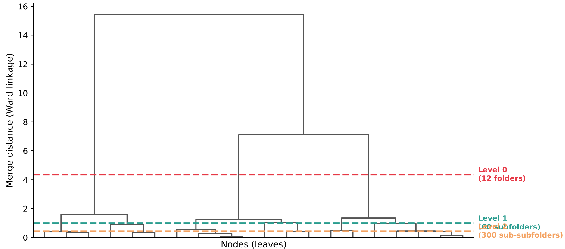
Dendrogram with three cuts producing the laminar hierarchy (illustrative; actual data has 5,798 nodes)
