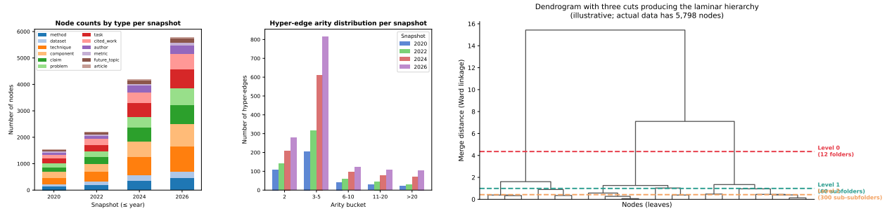
Figure 1: Left: node counts by type and hyper-edge arity distribution per snapshot. Right: illustrative dendrogram — three horizontal cuts yield the three hierarchy levels (12 / 60 / 300 clusters); actual data has 5,798 leaves.
