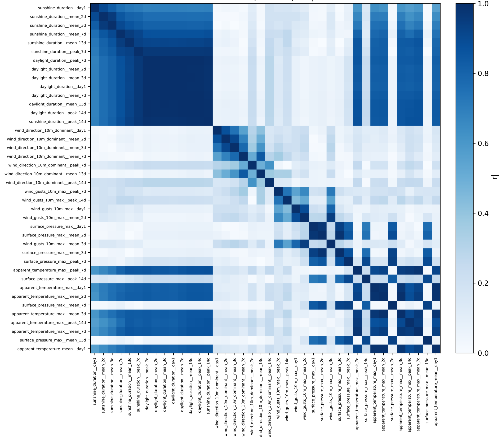
Weather correlation matrix (absolute) - top variance features
