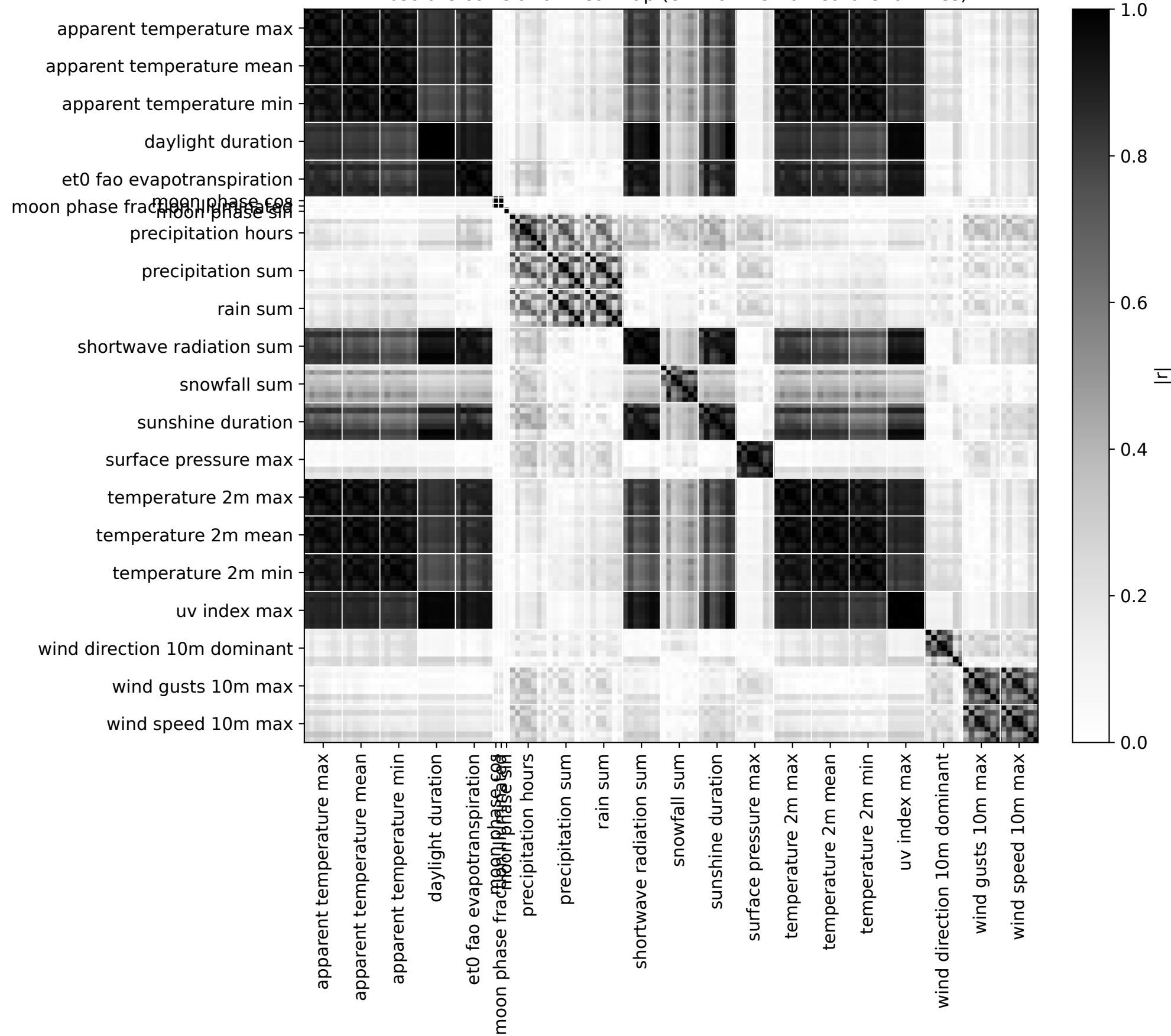
Absolute correlation heatmap (environmental feature families)
