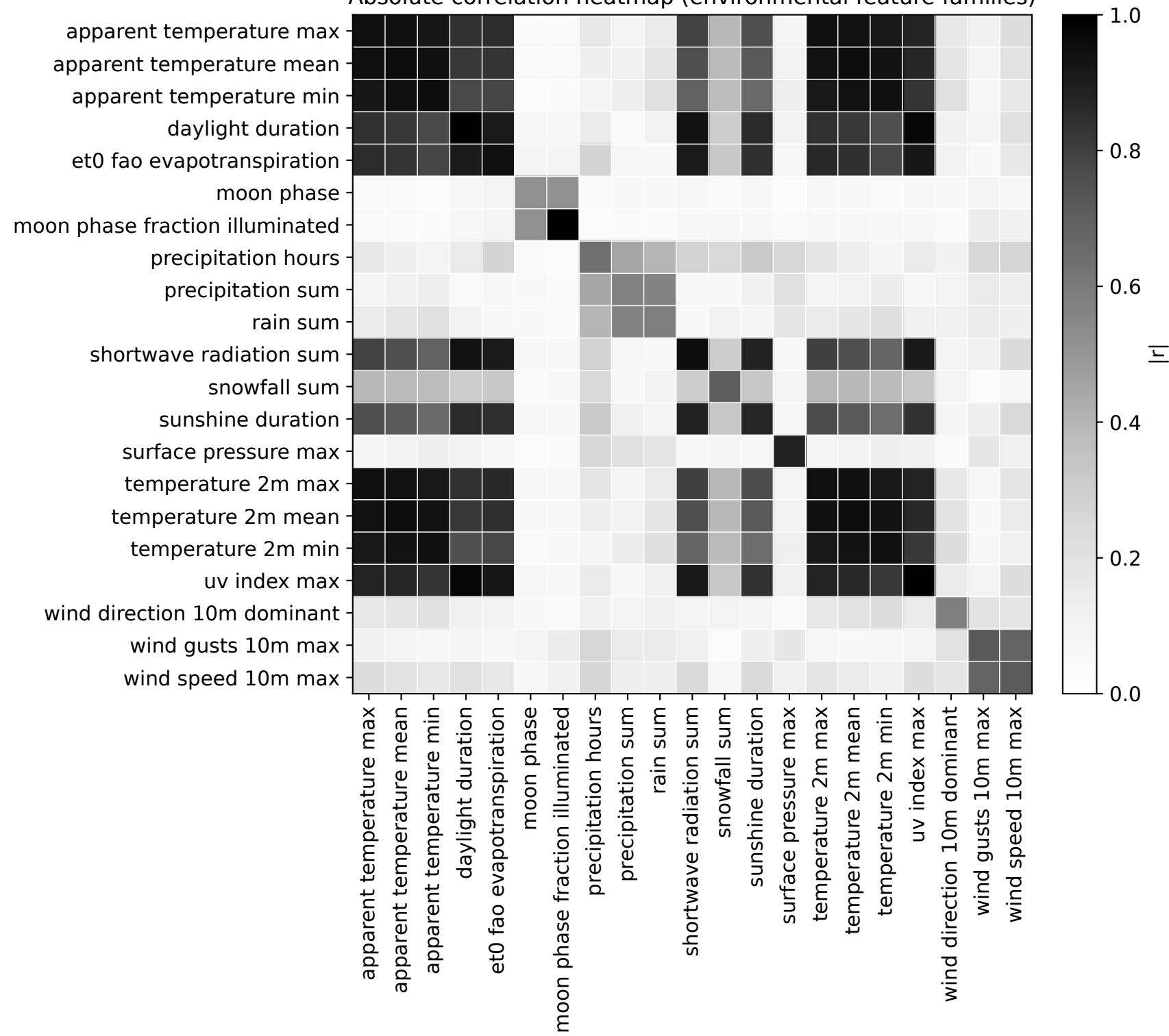
Absolute correlation heatmap (environmental feature families)
