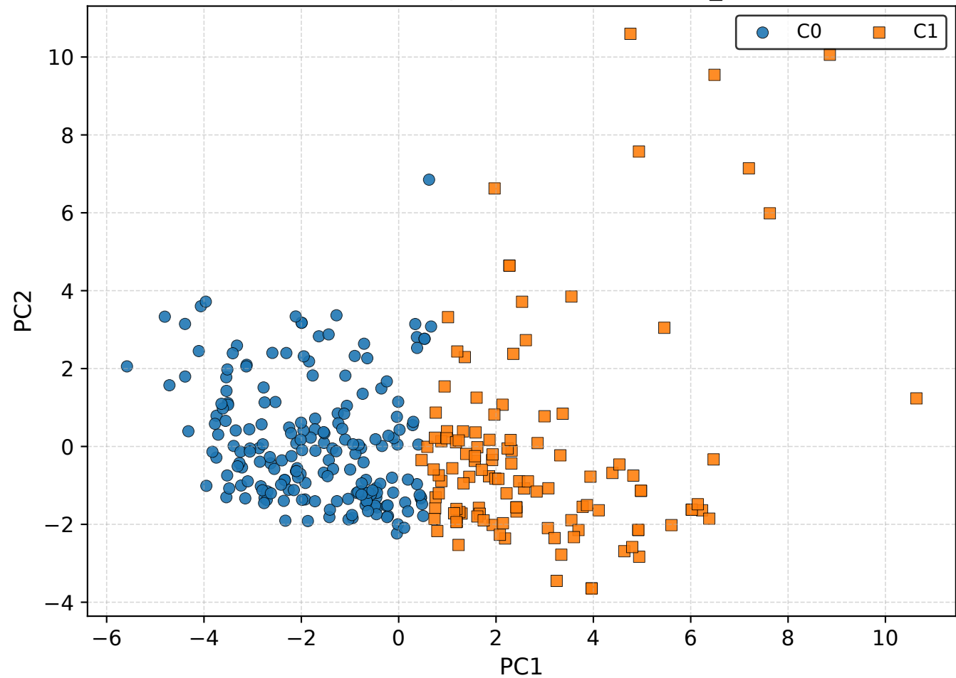
Environmental-only KMeans (Dfixed6, k_best=2)
