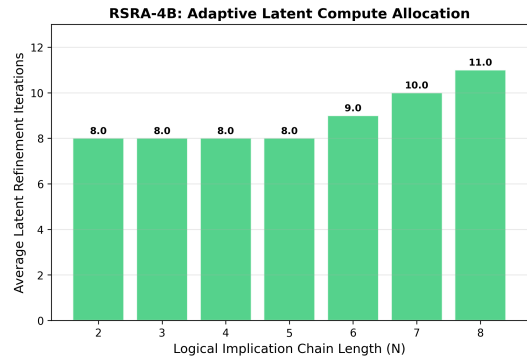
Figure 4: RSRA-4B Latent Iterations vs. Chain Length ( N ). The block dynamically allocates more iterations for complex reasoning steps, proving the effectiveness of our Banach-contraction-guided checker-verifier loop.
