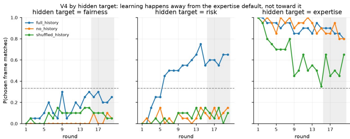
Figure 4. V4, by the partner's type: late held-out match with full history, no history, and shuffled history. Learning is largest where the default frame is weakest.
