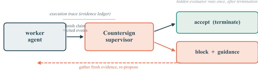
Figure 1: The supervision loop. The worker proposes termination with cited evidence; Countersign audits the claim against the execution trace and either accepts it or blocks it with a specific deficiency, after which the worker gathers fresh evidence and re-proposes. The hidden evaluator that determines correctness runs once, after termination, and is never consulted by the supervisor.
