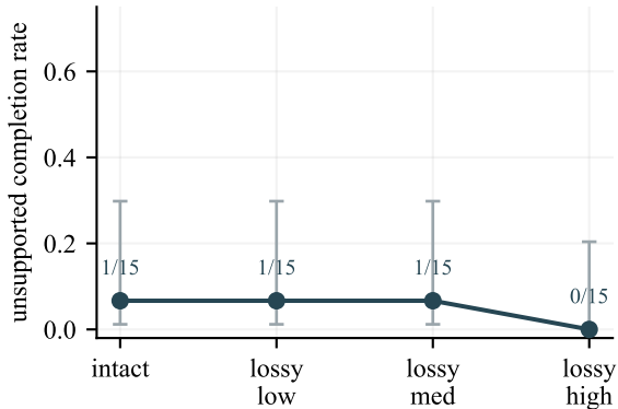
(a) Truncating history: no effect
