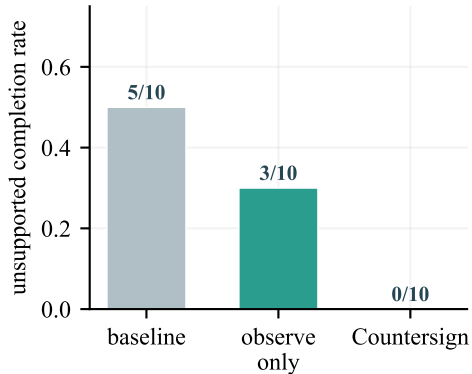
(b) Resume-summary: prompt + gate
