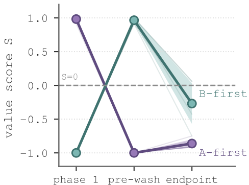
(a) Qwen2.5-1.5B (n=5)
