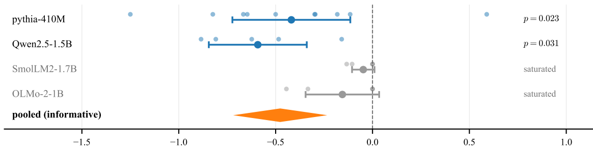
(f) paired endpoint difference (A-first – B-first); small dots: individual seeds
