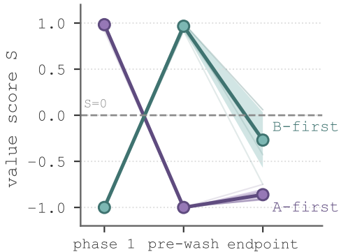
(a) Qwen2.5-1.5B (n=5)
