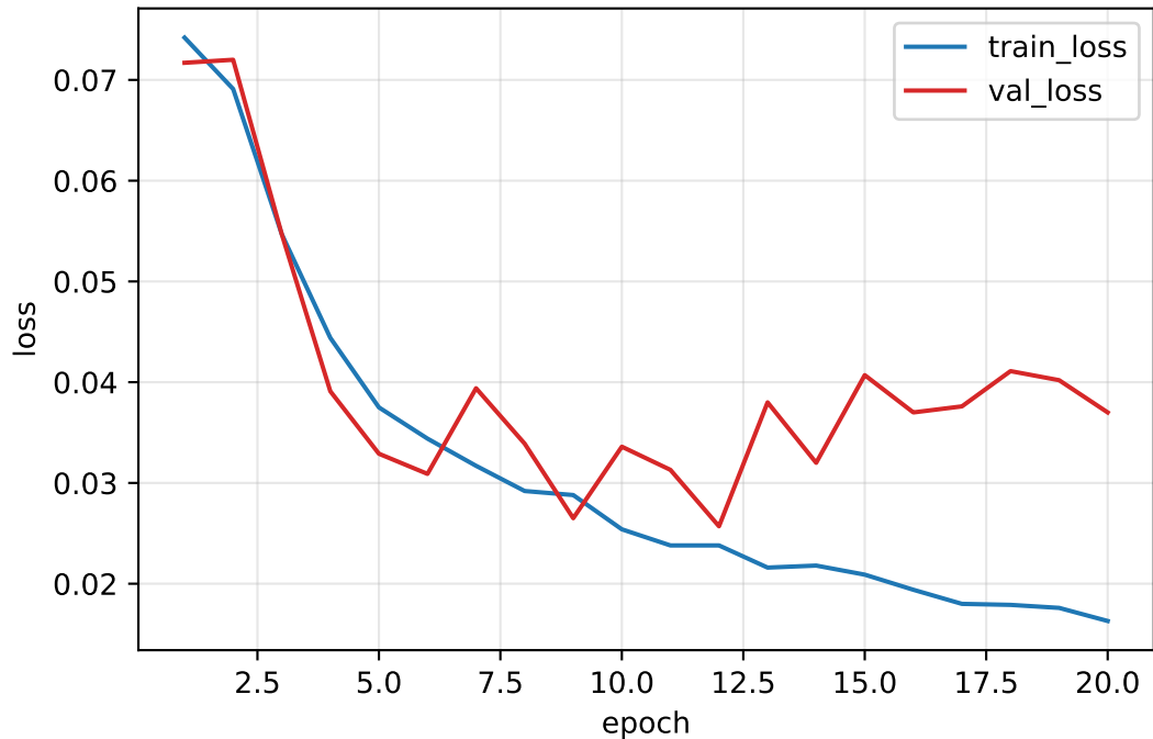
cnn1d_seed42: focal-loss
