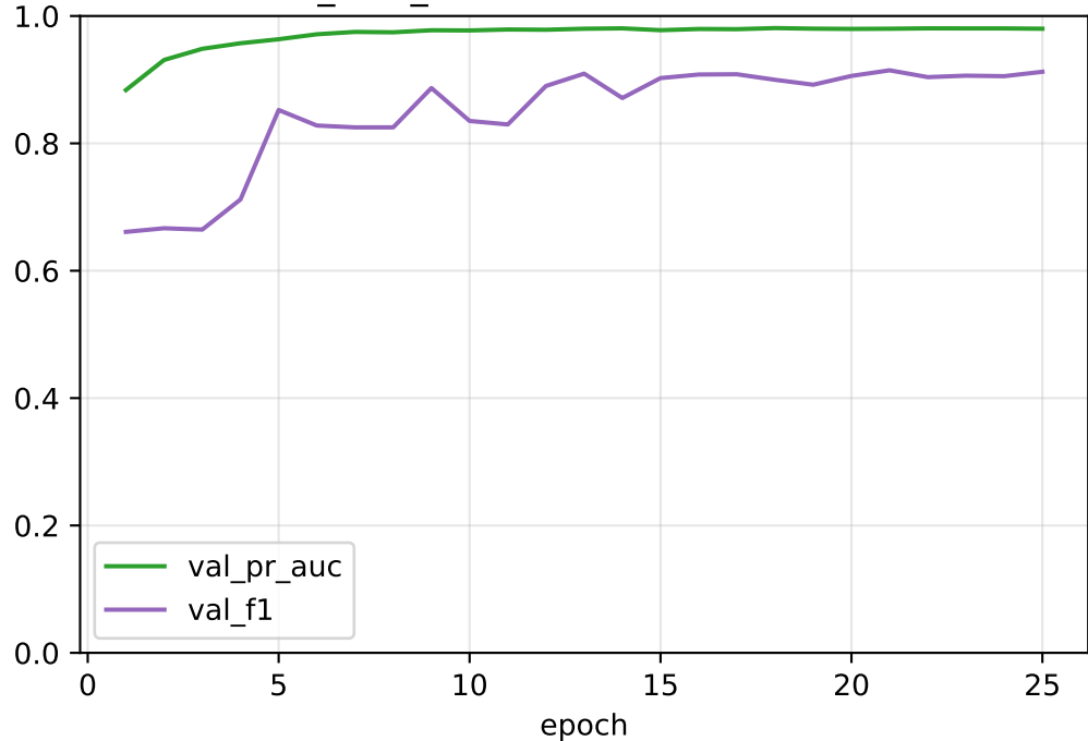
cnn_lstm_seed123: validation metrics
