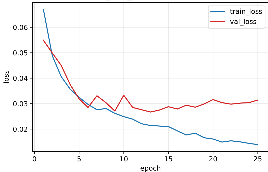
cnn_lstm_seed123: focal-loss
