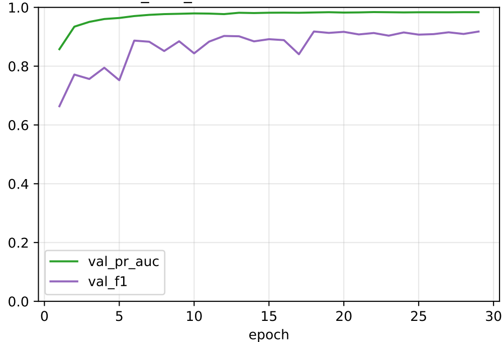
cnn_lstm_seed2024: validation metrics
