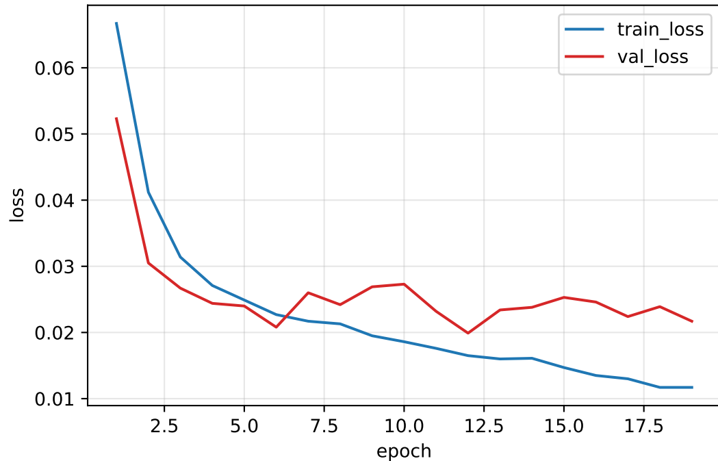
gru_seed42: focal-loss
