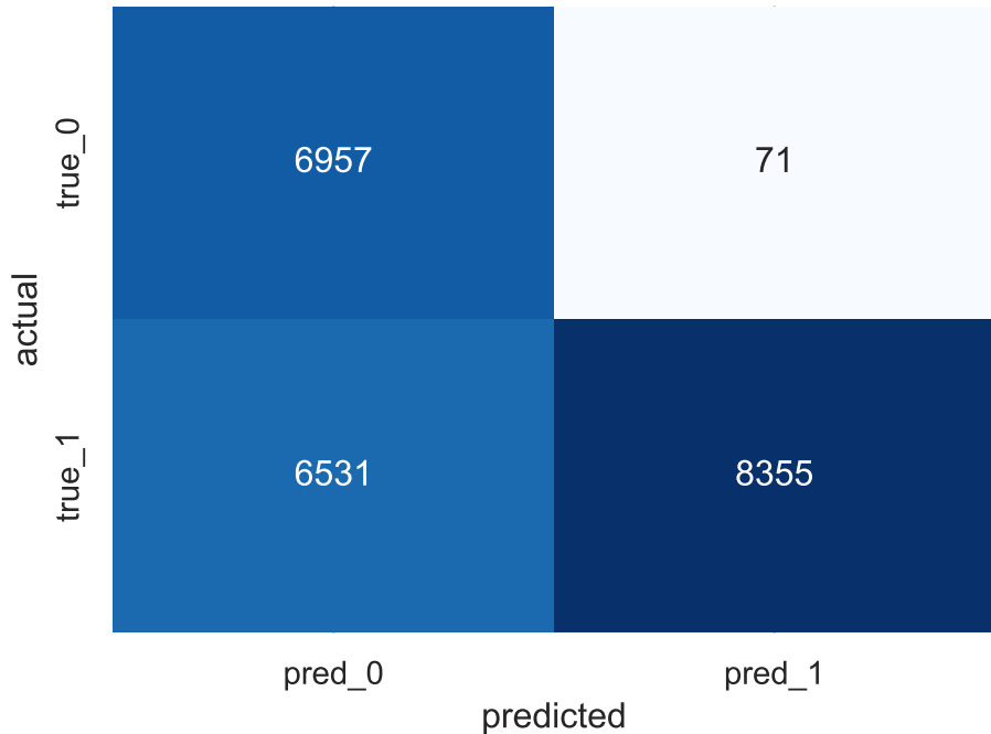
CNN-LSTM confusion matrix (test)
