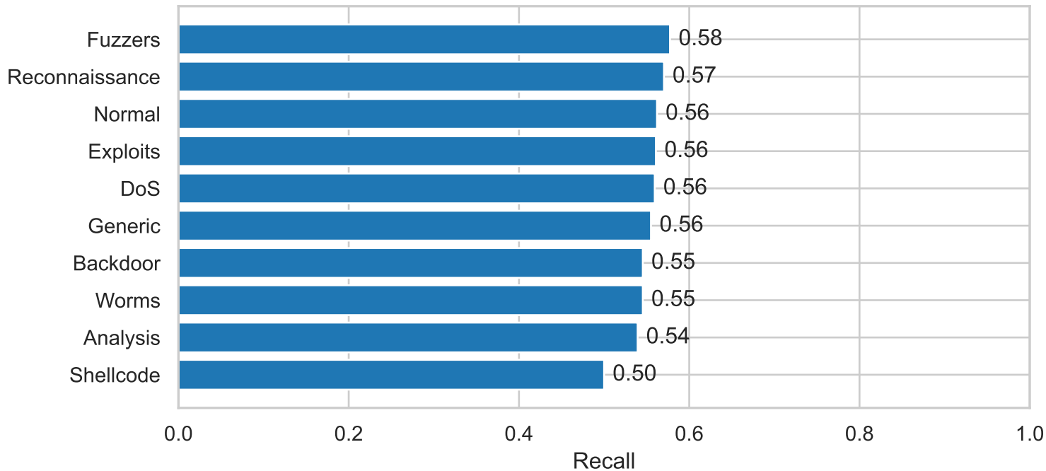
CNN-LSTM recall per attack_cat (test)
