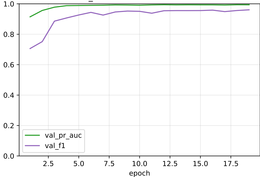
tcn_seed42: validation metrics
