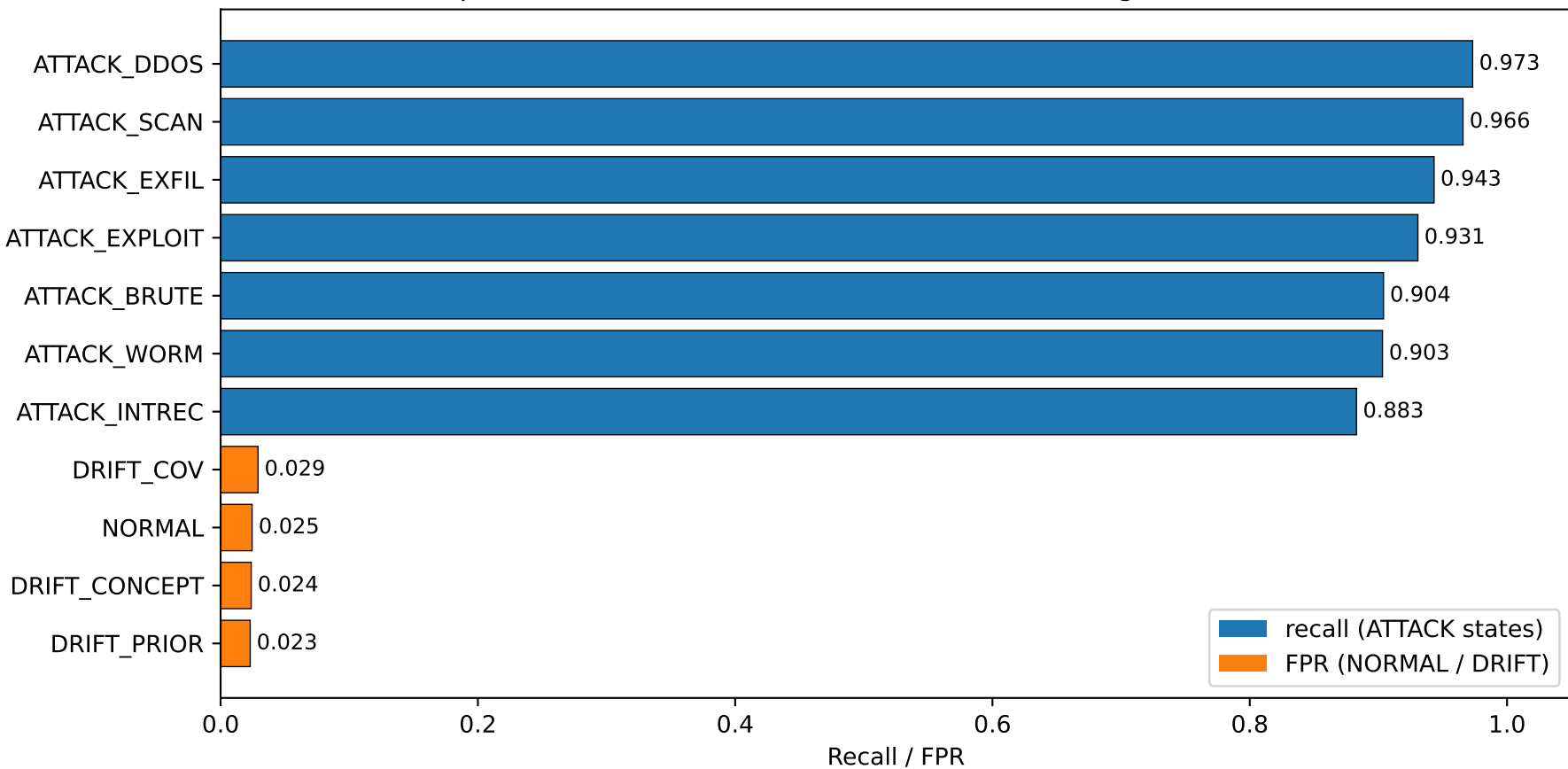
E4: per-state behaviour of CNN-LSTM under FSM agent (20 000 ticks)
