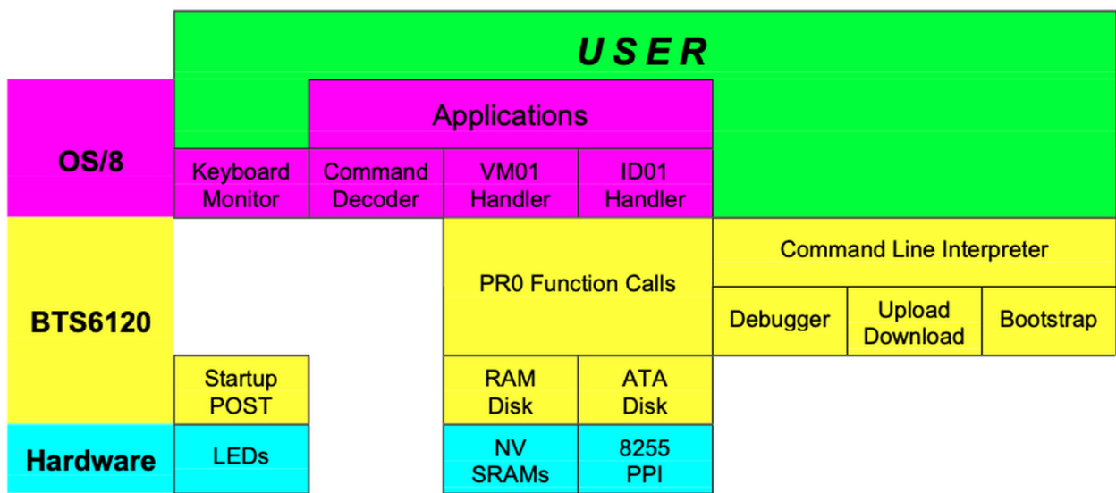
Figure 6 - SBC6120 Software Architecture
