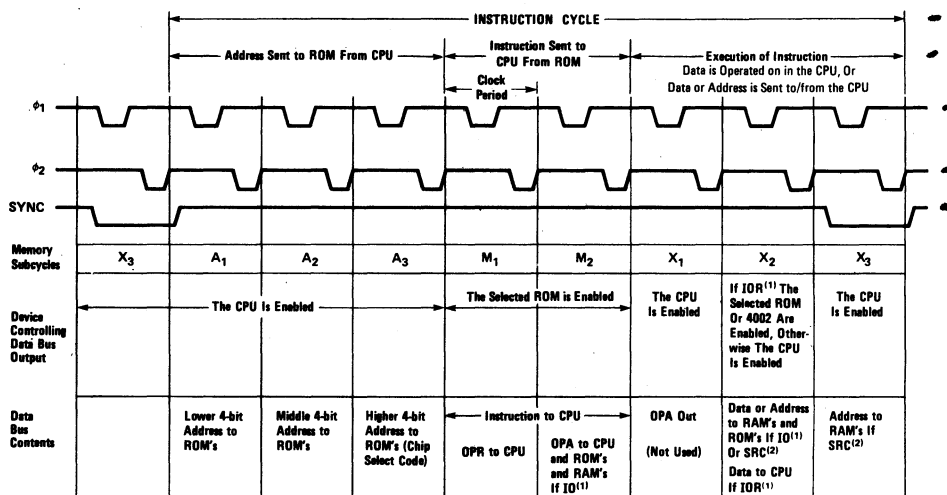
Figure 1-2. 4004 Basic Instruction Cycle.
