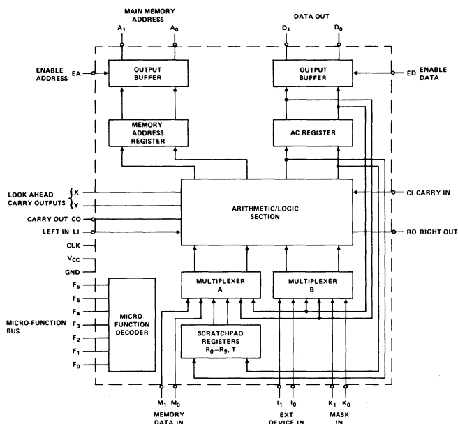
Figure 2. 3002 Block Diagram
