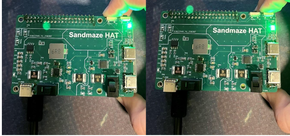
Figure 1: Test T-RB3-0/1
