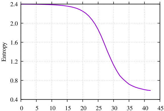
Entropy Decay
