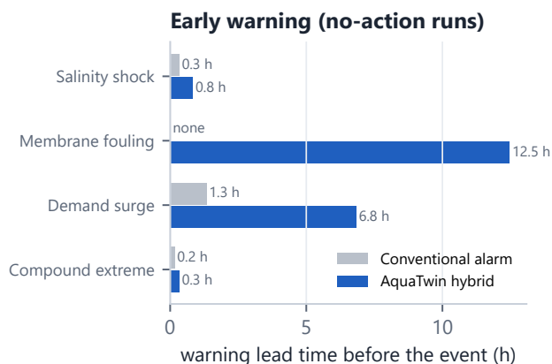
Figure 8. Warning lead time before the first critical event (no-action runs, mean of seeds). Simulated.
