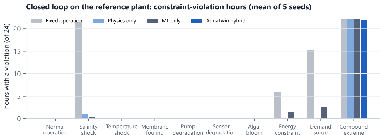
Figure 4. Hours with any constraint violation on the true plant, mean of five seeds. Simulated.
