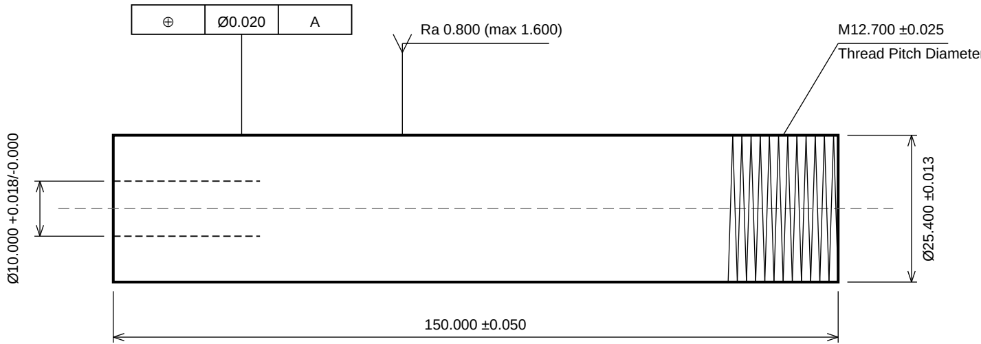
SIDE VIEW
