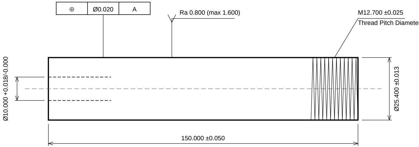
SIDE VIEW
