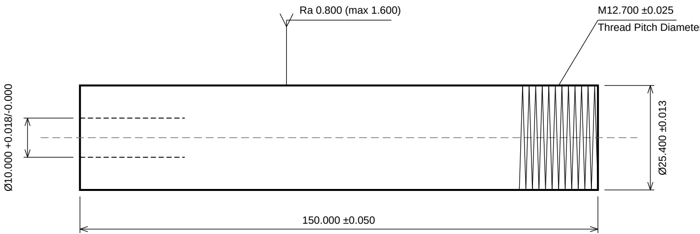
SIDE VIEW
