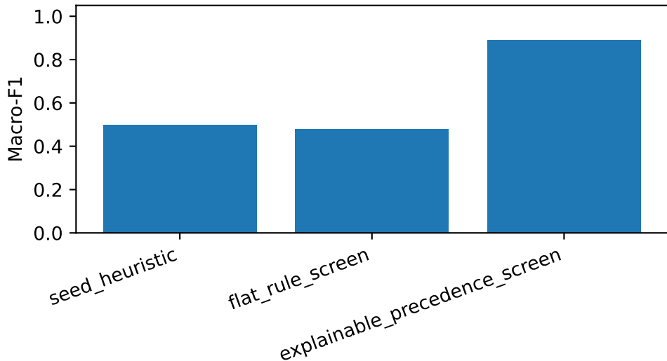
Macro-F1 by screening condition
