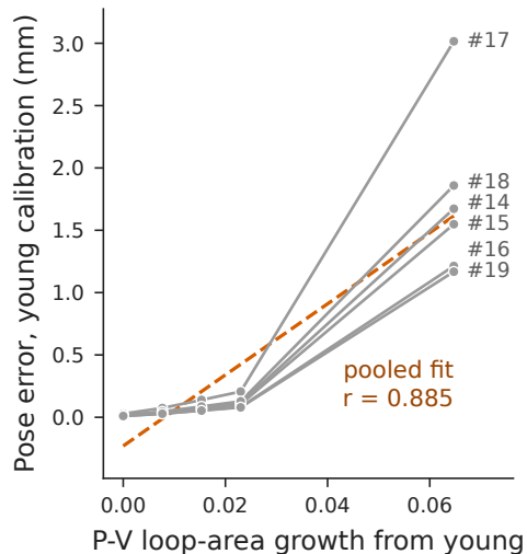
a Six actuators share one indicator trajectory; only pose error differs
