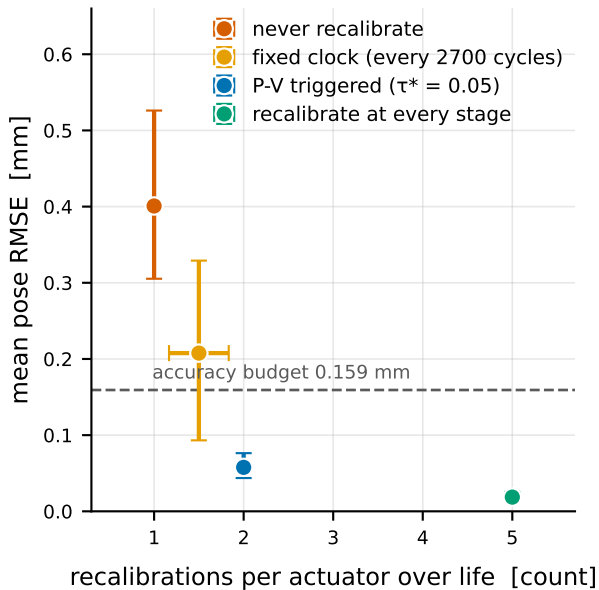
a Only the fixed-clock baseline varies across actuators
