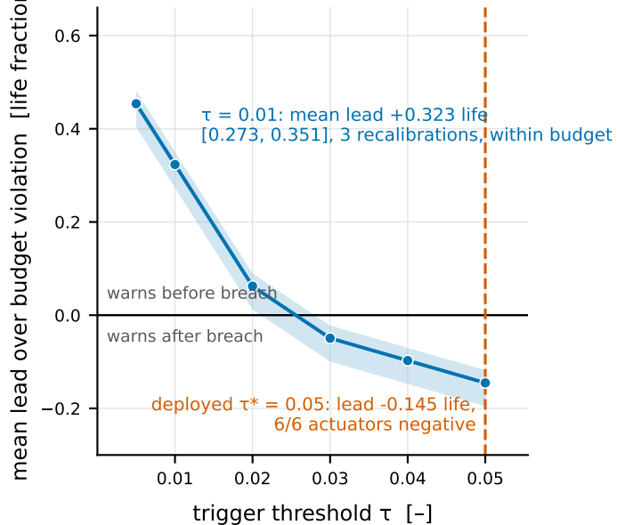
b The deployed threshold fires after the error budget is already breached
