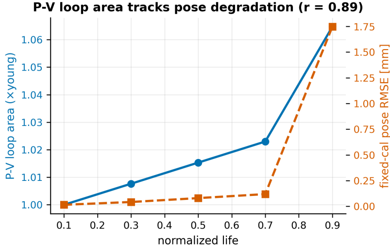
Figure 3. Observable P-V loop-area growth (left axis) tracks fixed-calibration pose error (right axis) over life on held-out actuators; bootstrap r = 0.885 , 95% CI [0.835, 0.958] . The deployed threshold does not provide positive temporal lead, but lower thresholds define a lead-vs-recalibration frontier.
