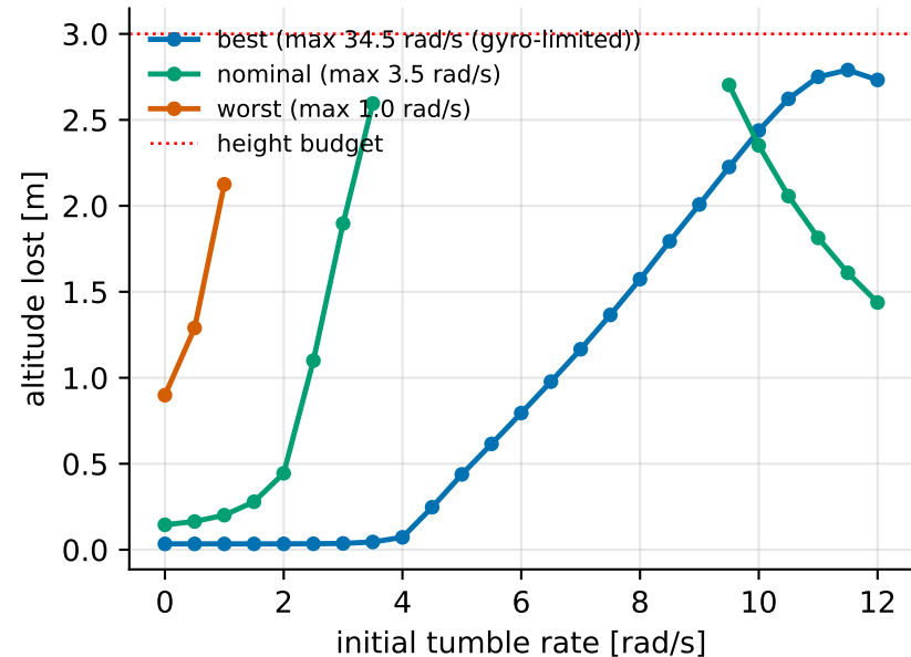
Altitude lost vs tumble rate
