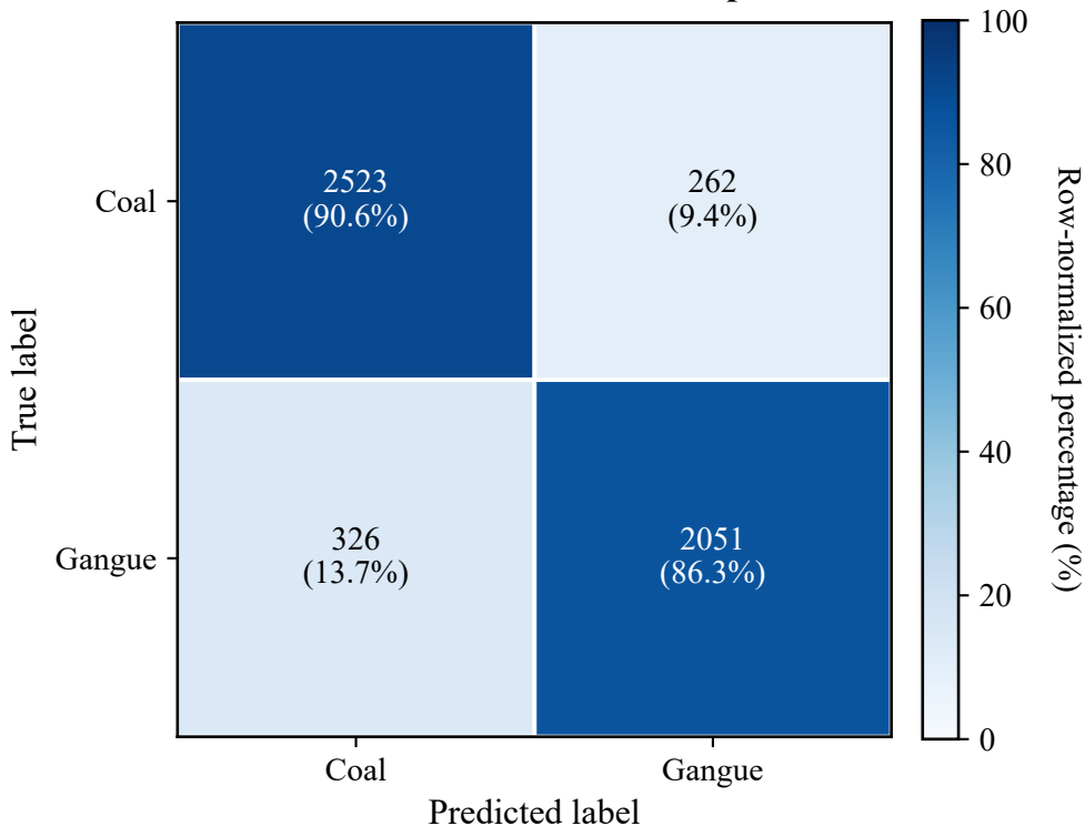
Confusion matrix under the P4 protocol
