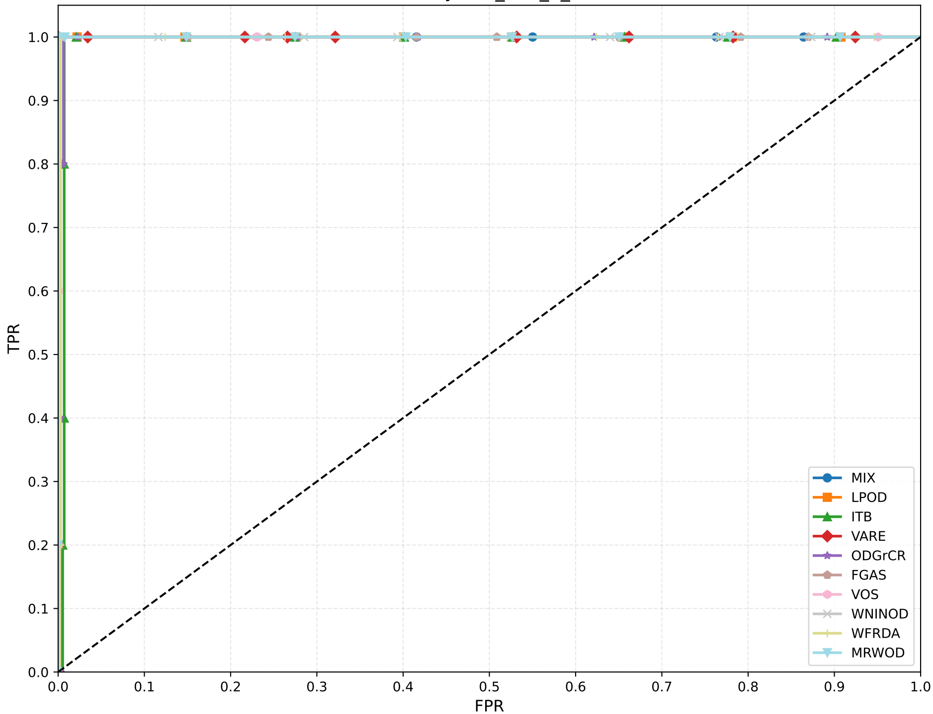
ROC Curve: yeast_ERL_5_variant1
