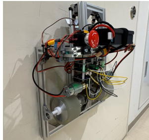
Fig. 2 Appearance of scraper-integrated robot
