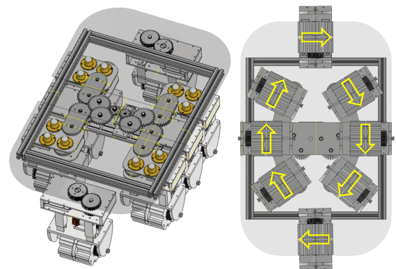
Fig. 1 machine blueprint
