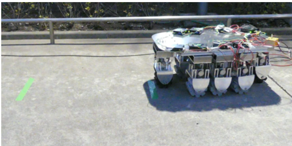
Fig. 7.2 Driving experiment on concrete
