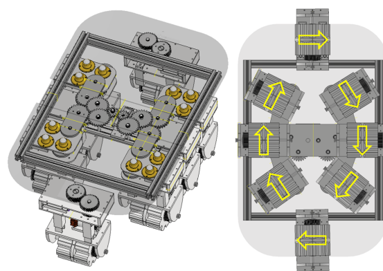
Fig. 1 machine blueprint
