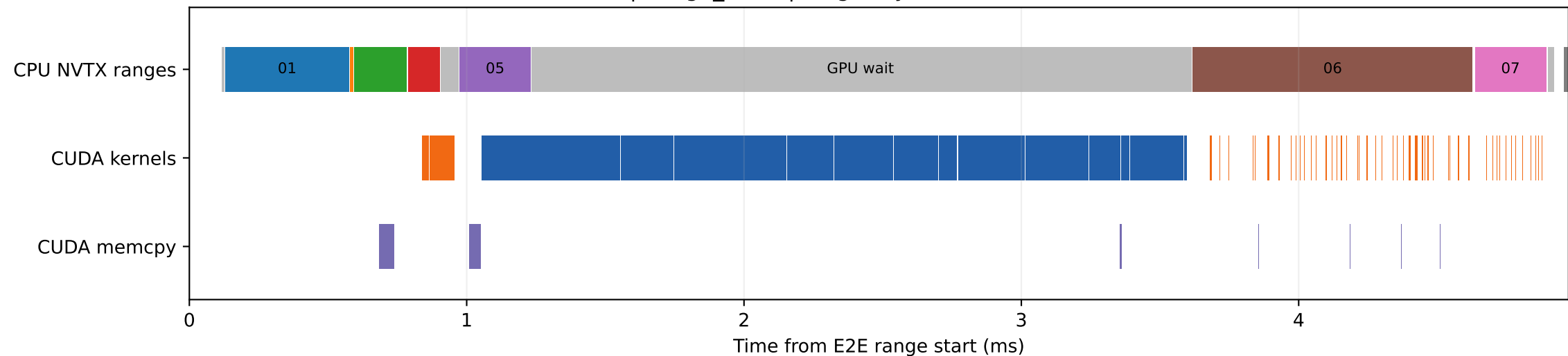
KITTI | image_0028 | Nsight Systems measured timeline
