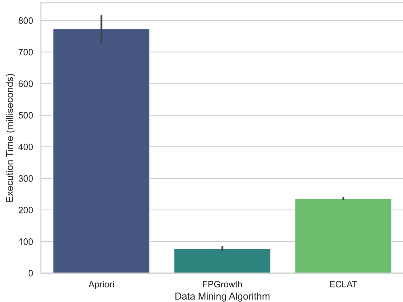
Algorithm Execution Time Comparison
