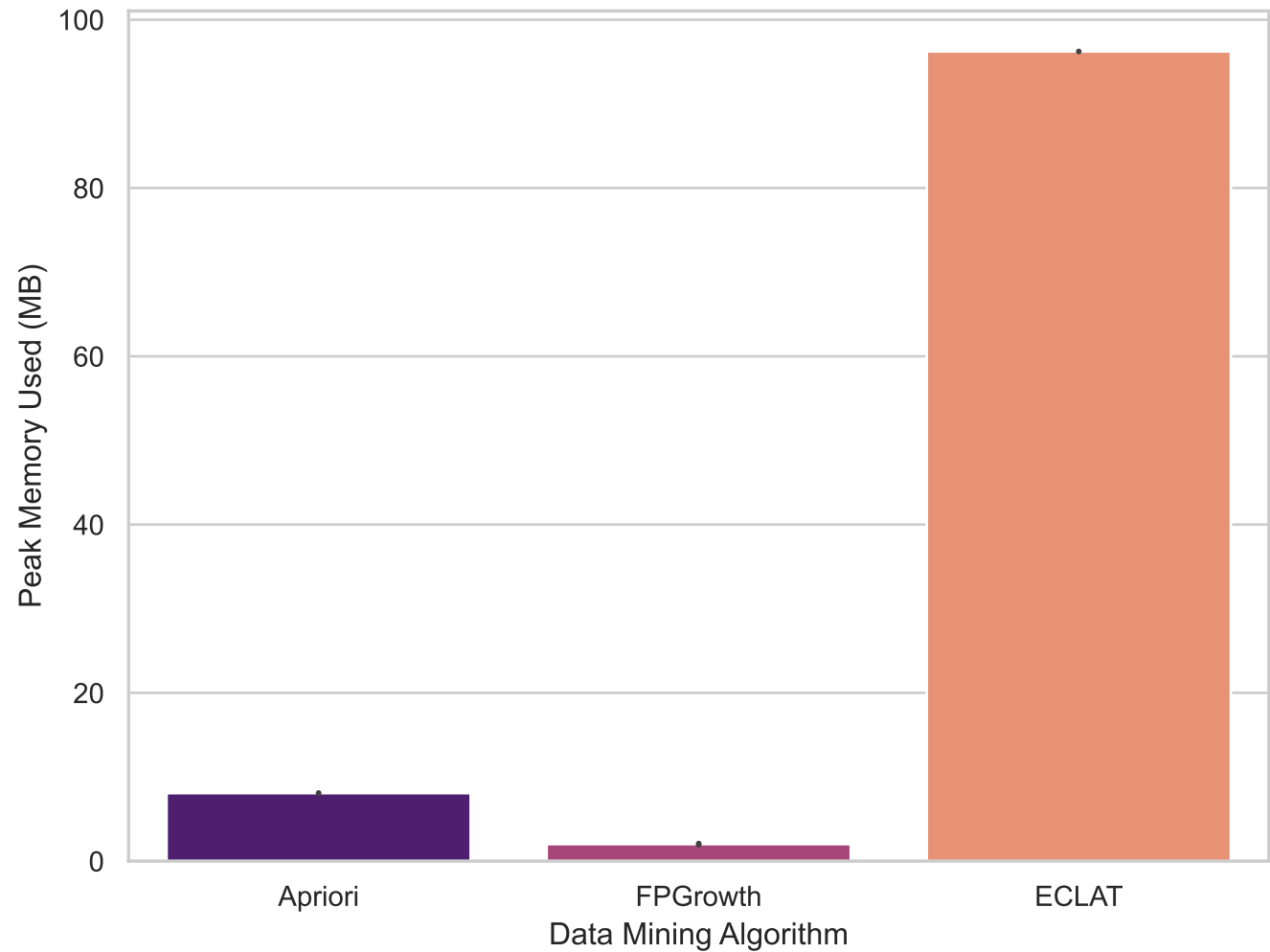
Algorithm Memory Consumption Comparison
