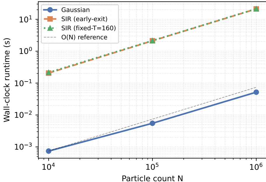
Sequential Runtime vs Particle Count
