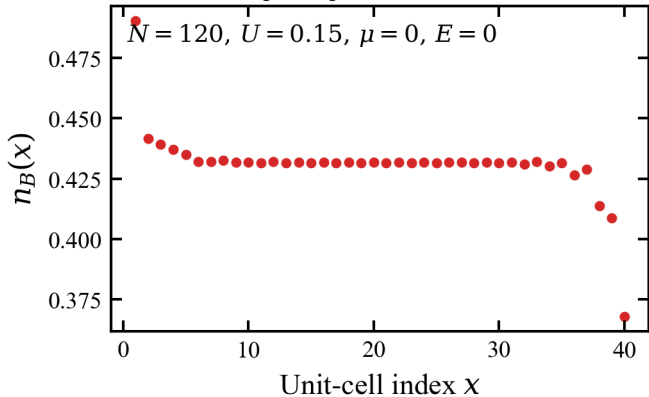
Occupation profile of the B orbital
